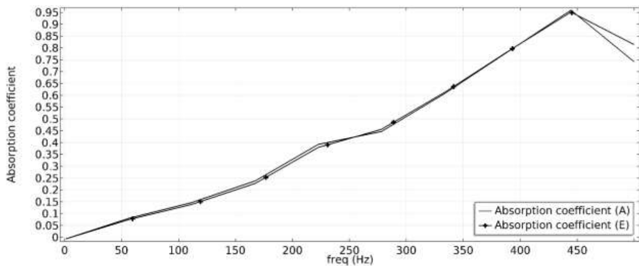
Fig. 7. Comparisons of two designs (shapes) of “A” and “E”
