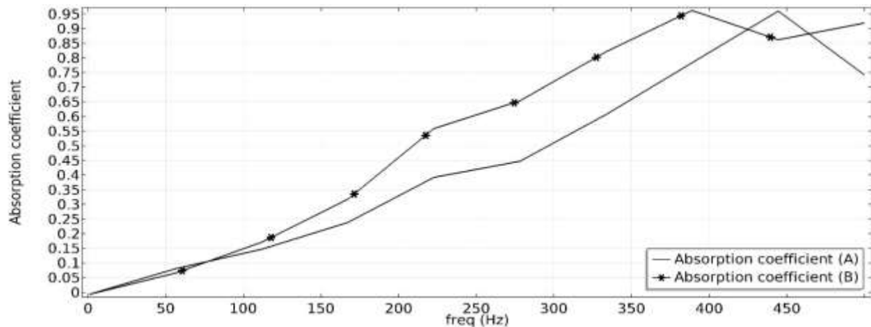
Fig. 4. Comparisons of two designs (shapes) of “A” and “B”
