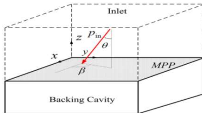
Fig. 1. Theoretical model of the MPP absorber
